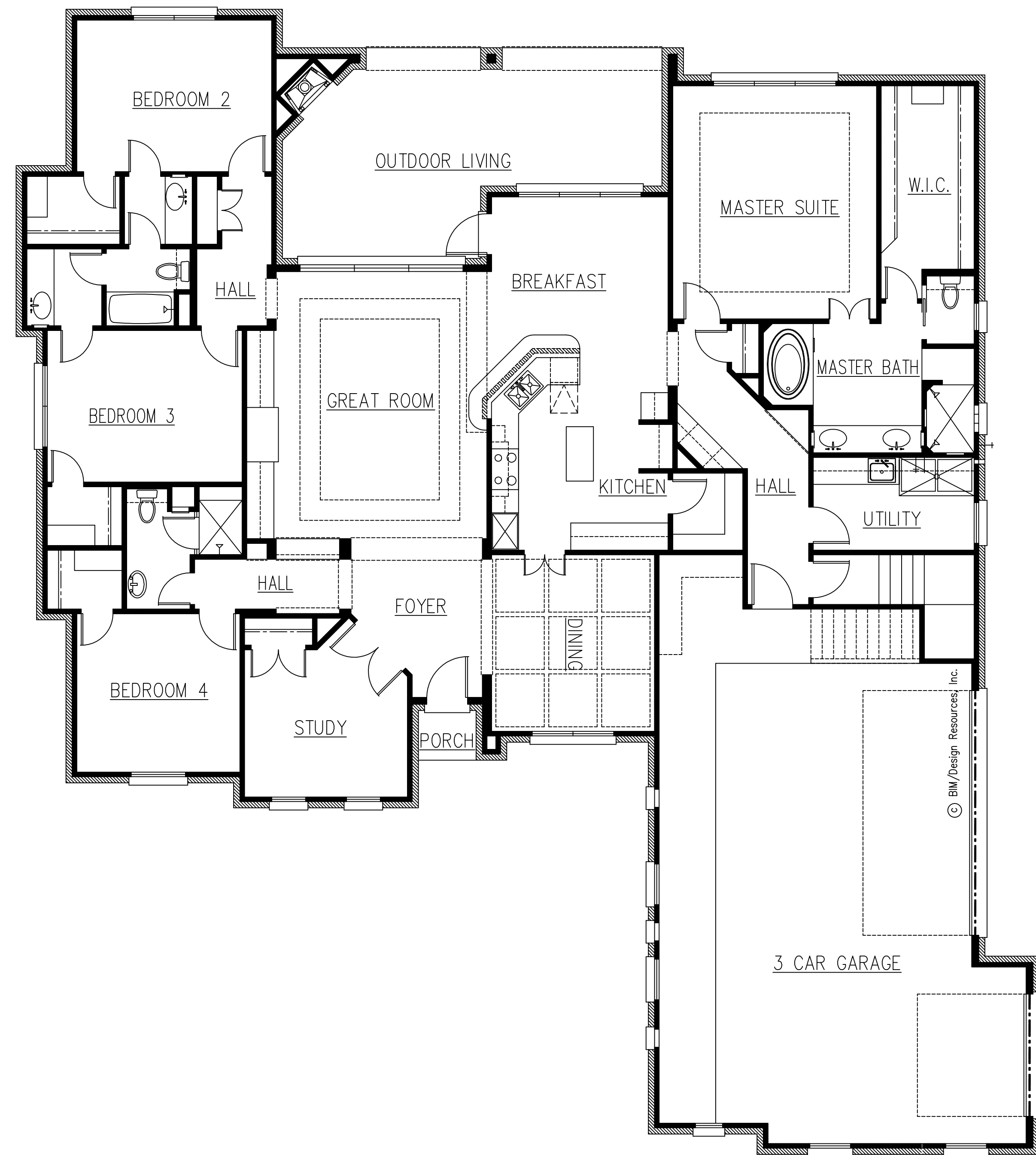
FIRST FLOOR
